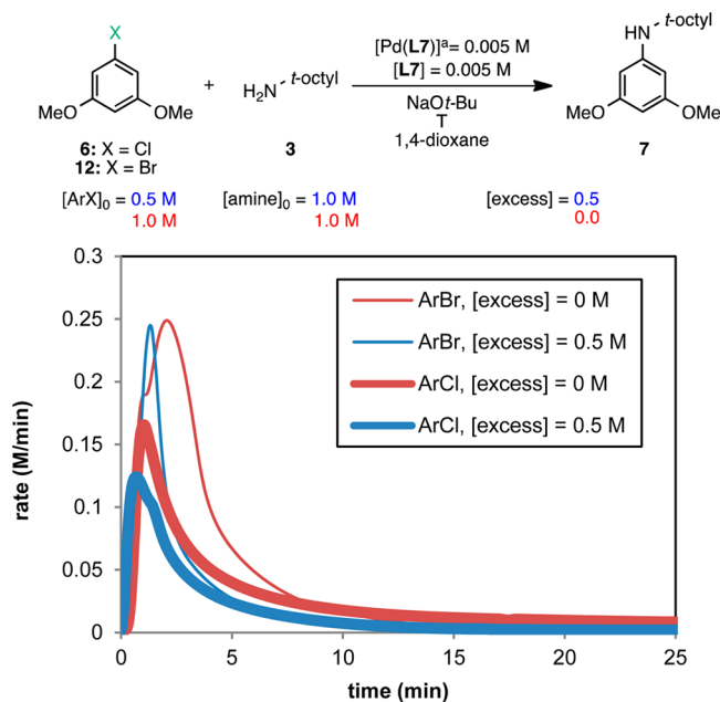
Figure 6. Temporal reaction rate profiles for the reaction of amine 3 (1.0 M) and ArCl 6 or ArBr 12 (concentrations defined by [excess] given in legend; see eq 1). Reaction at 70 °C for ArCl and 60 °C for ArBr in 1,4-dioxane. Note a: Pd(L7) is an oxidative addition complex generated in situ from (COD)Pd(CH 2 TMS) 2 , L7, and 12 (see the Supporting Information for details).
